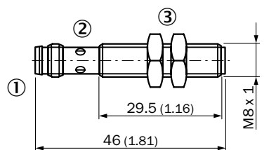
MM08, connector, standard sensing range
