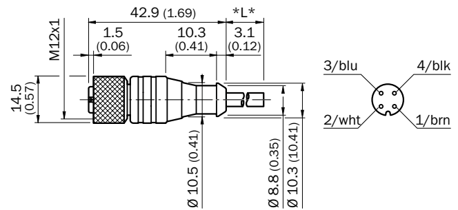
DOL-1204-G05MA
