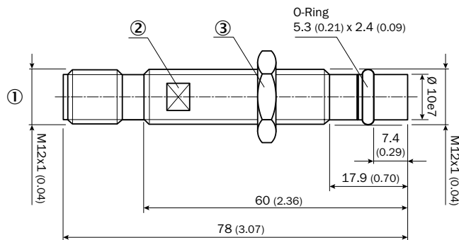
IMP12-xxxxxxxD, 78 mm
