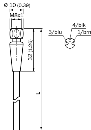
DOL-0803-GxxMRN
