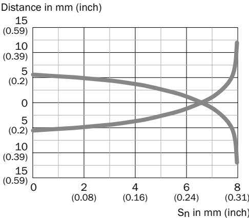
IMF12, non-flush installation
