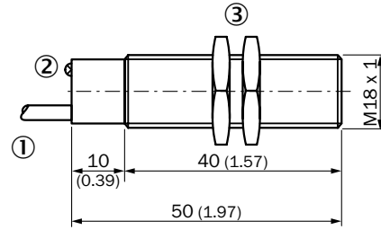
MM18 Namur, cable
