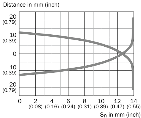
IMB30, flush installation
