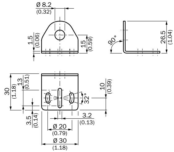
BEF-WN-M12 / BEF-WN-M12N
