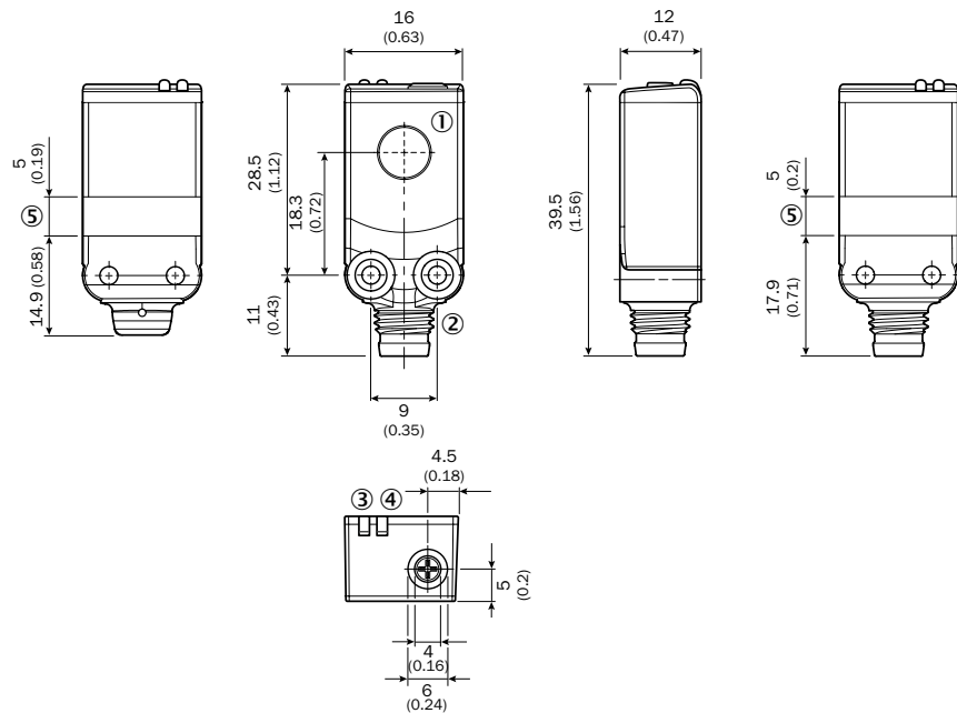
CQ4, connector
