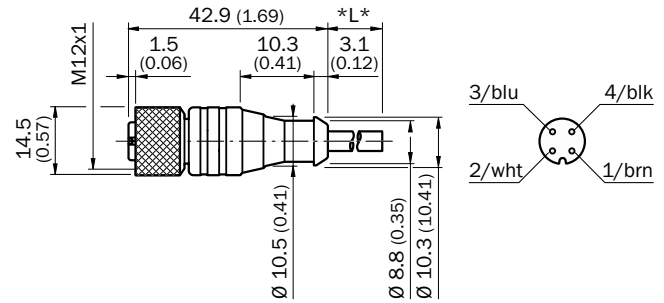
DOL-1204-GxxM
