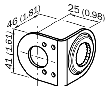
BEF-KHS-H01
