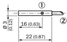
IH03, standard-body, flush, cable
