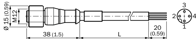
DOL-1204-GxxMNI
