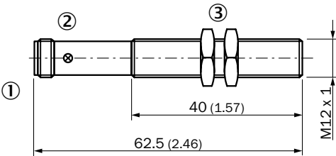
MM12 Namur, connector
