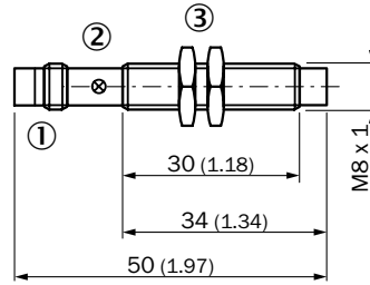
IME08 standard, male connector, non-flush
