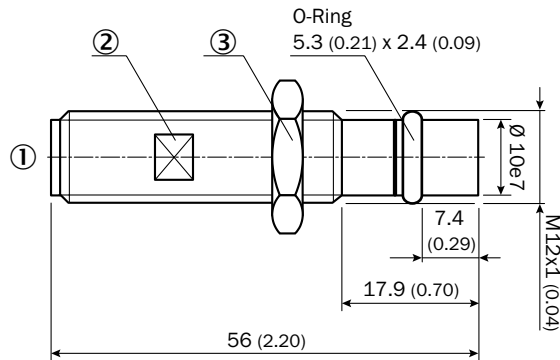
IMP12-xxxxxxxB, 56 mm
