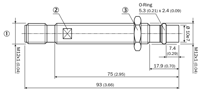
IMP12-xxxxxxxF, 93 mm
