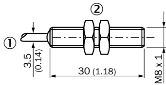
IMN08 Namur, flush
