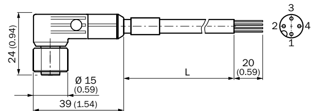
DOL-1204-LxxMNI
