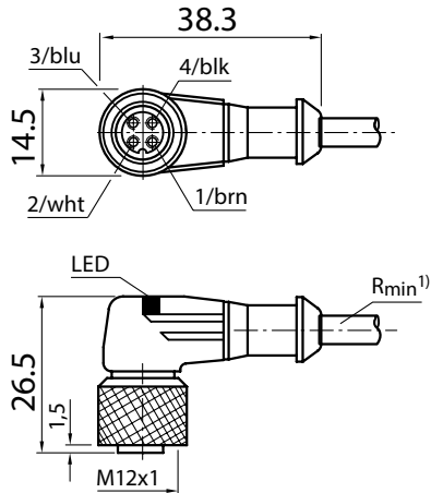
DOL-1204-GxxMRN / DOL-1205-GxxMRN
