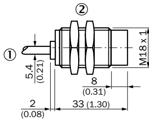
IM18 Namur, non flush
