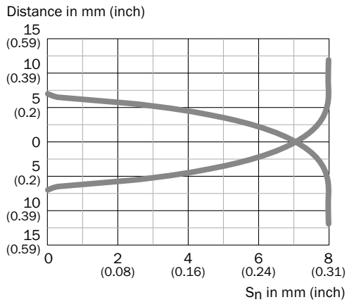
IMB18, flush installation
