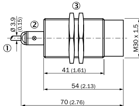
IME30 Standard, cable, non-flush
