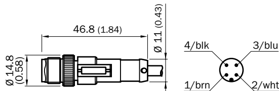
STL-1204-GxxMC
