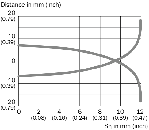
IMF18, non-flush installation
