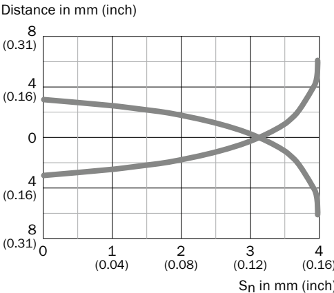
IMF12, flush installation
