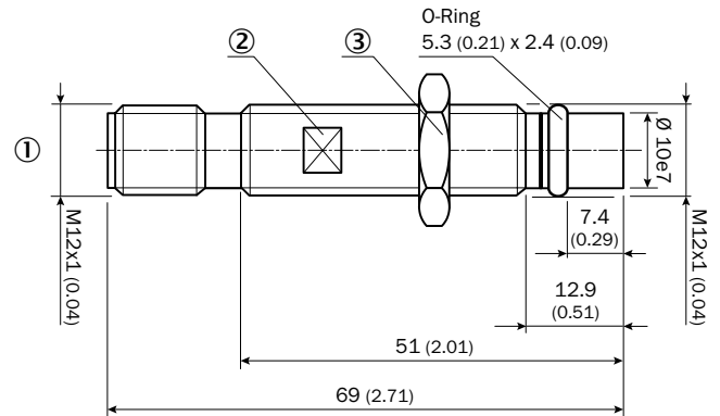
IMP12-xxxxxxxC, 69 mm
