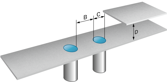
Flush installation
