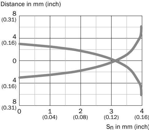
IMF08, non-flush installation
