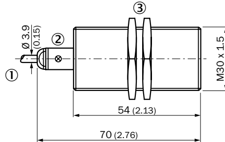
IME30 Standard, cable, flush
