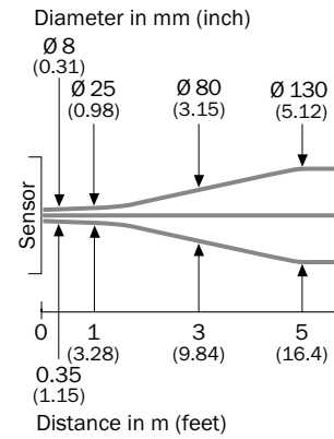
GL6 Inox, visible red light, 5 m
