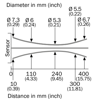
GTE6 Inox, visible red light, 250 mm
