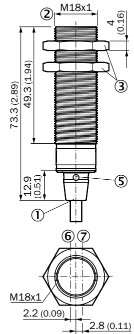
GRTE18, GRL18, GRSE18 Inox, cable, no adjustment possibility
