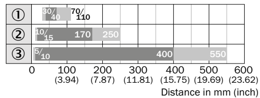
GRTE18(S) Inox, 400 mm
