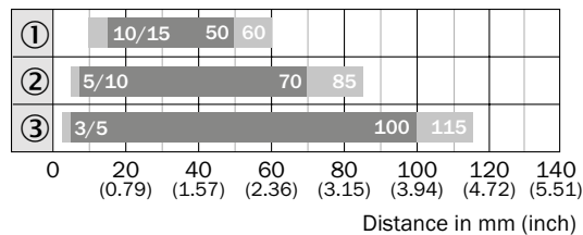
GRTE18(S) Inox, 100 mm
