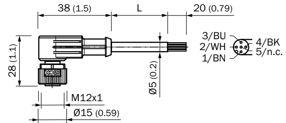
YG2A14-xxxVB3XLEAX, PVC, YG2A24-xxxVB4XLEAX, PVC
