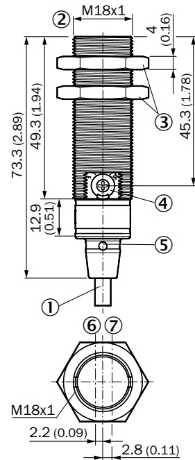
GRTE18, GRL18, GRSE18 Inox, cable, potentiometer, 270°
