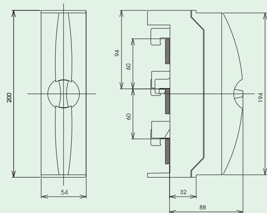
BBA-TP3/50
