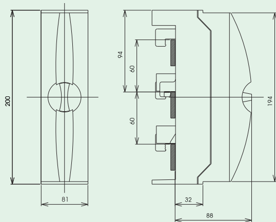
BBA-TP3/120
